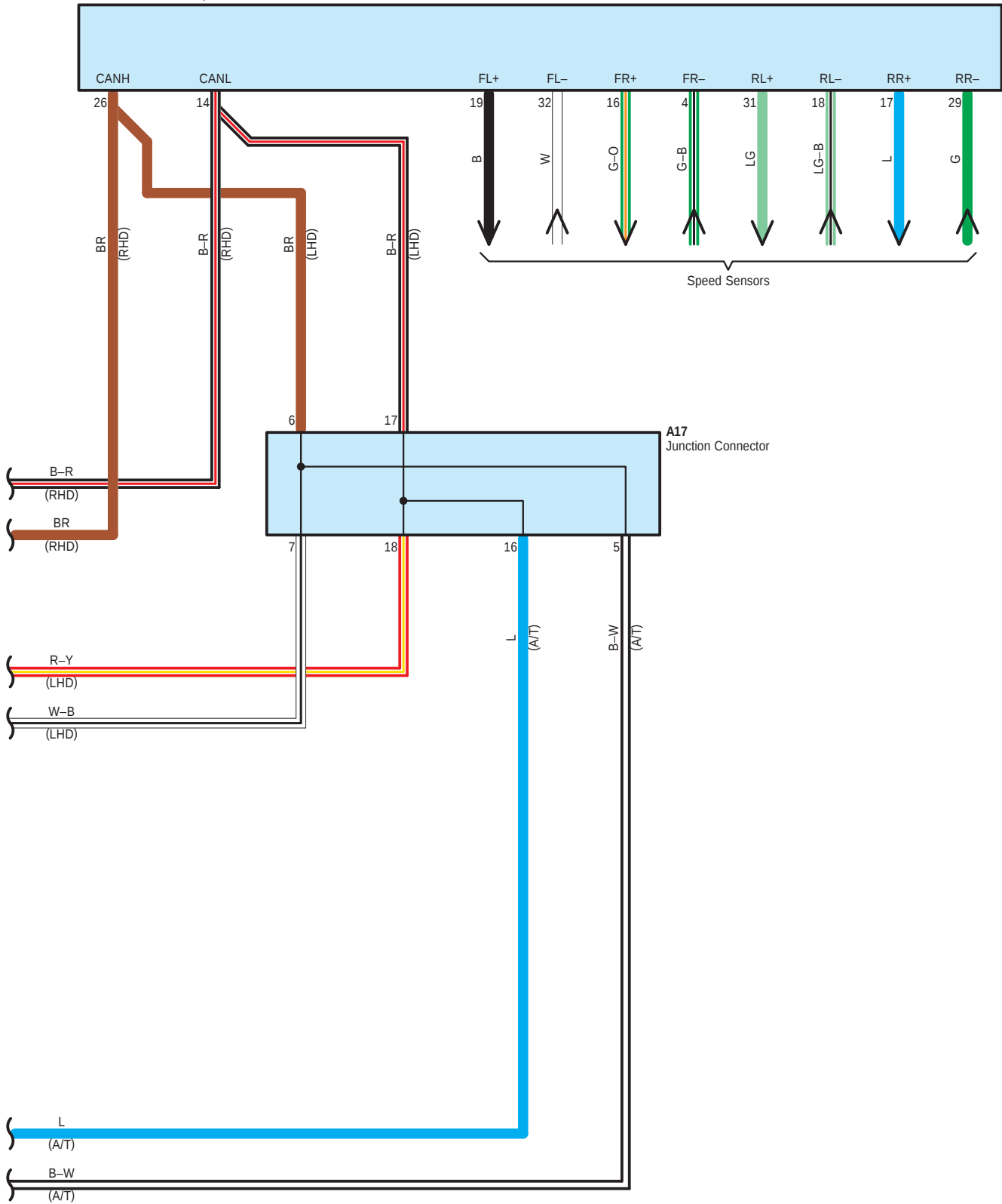
A5 Brake Actuator Assembly
